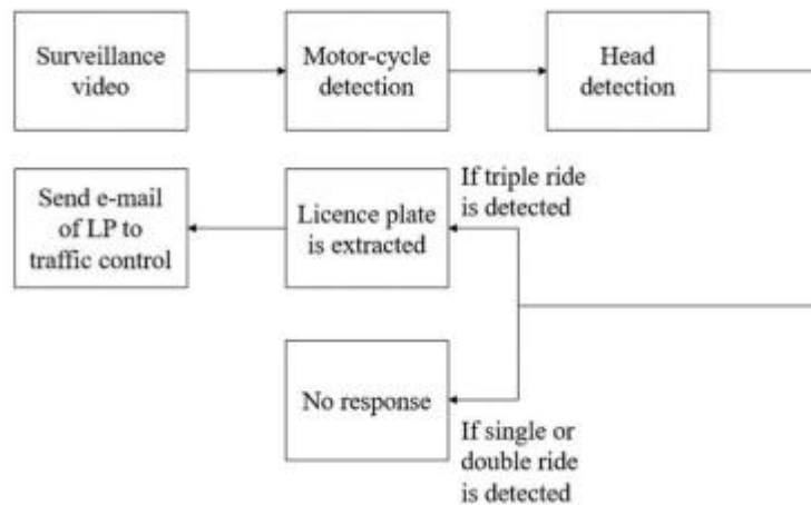
Fig 3. Block Diagram of the System
