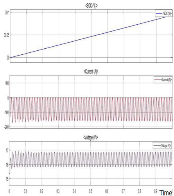
Fig.5. Charging of EV2
