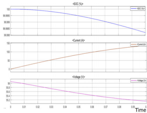
Fig.4. EV1 discharging.
