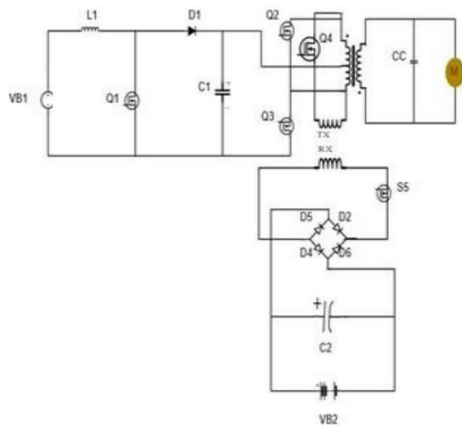
Fig.2. Circuit diagram.
