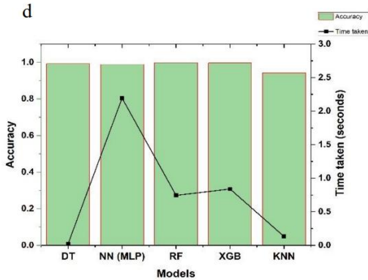
FIGURE 4 Comparison of accuracy and time taken for models execution for 70:30 ratio. Panels a, b, c and d represents Coastal, Forest, Transitional and Savannah zones respectively
