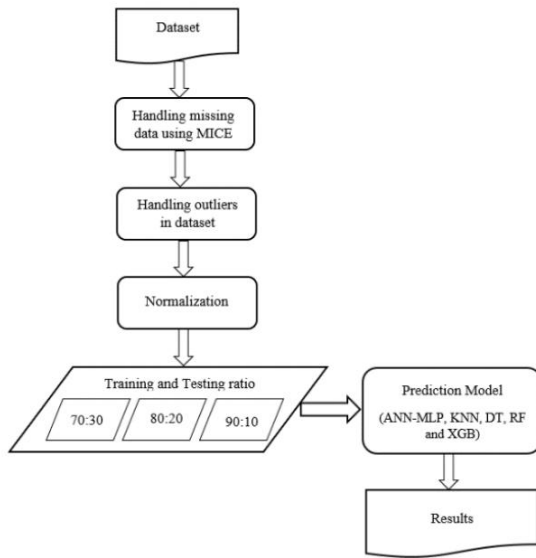
FIGURE 2. Classification framework.
