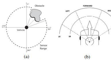
Fig. 4. In (a) we see LIDAR detecting an obstacle. In (b) we categorize collected data based on measurement location.
