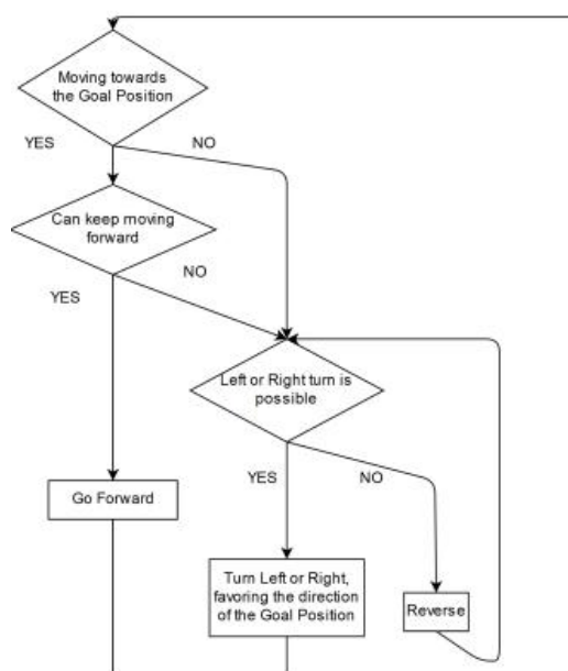
Fig. 5. Our Decision Making Algorithm.
